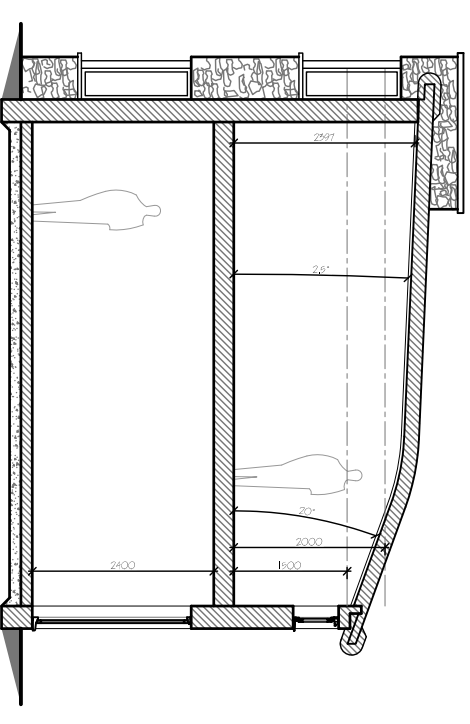
PROPOSED SECTION
